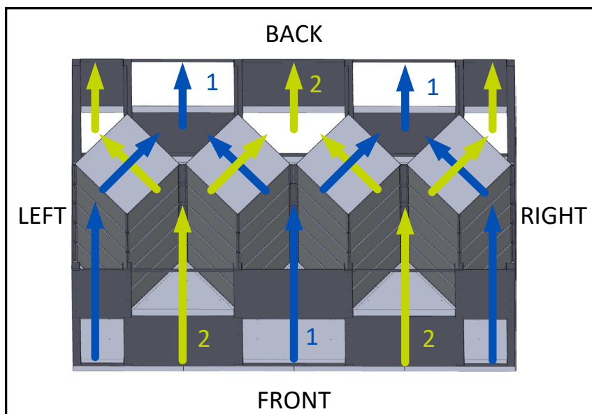
FIGURE 2.0.2 CROSSFLOW SAME SIDE ARRANGEMENT 2
