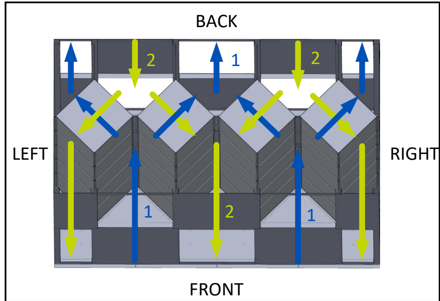
FIGURE 2.0.4 PARALLEL FLOW OPPOSITE SIDE ARRANGEMENT 3
