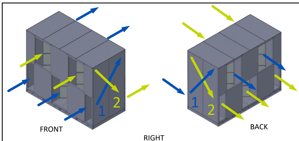
FIGURE 2.0.3 CROSSFLOW SAME SIDE ARRANGEMENT 2, SIDE VIEWS
