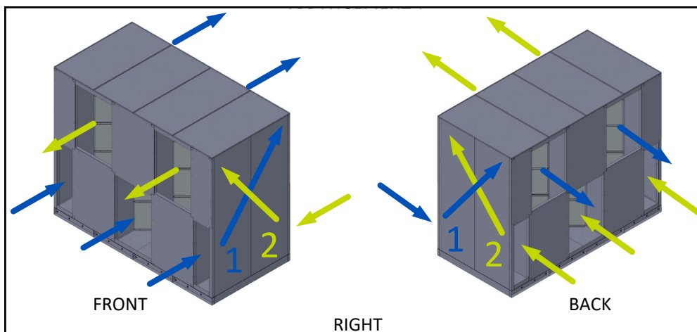
FIGURE 2.0.1 CROSSFLOW OPPOSITE SIDE ARRANGEMENT 1, SIDE VIEWS
