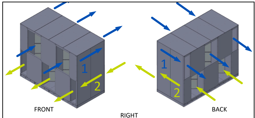
FIGURE 2.0.5 PARALLEL FLOW OPPOSITE SIDE ARRANGEMENT 3, SIDE VIEWS
