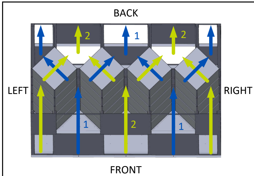
FIGURE 2.0.6 PARALLEL FLOW SAME SIDE ARRANGEMENT4
