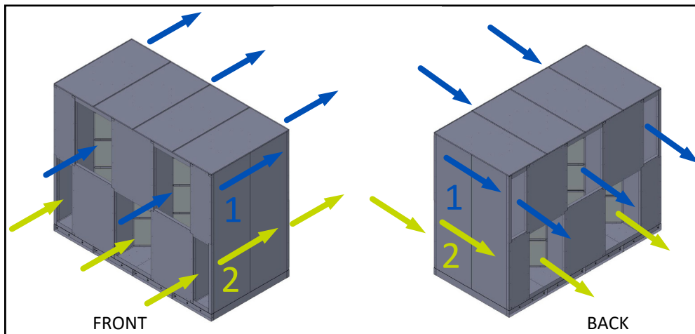
FIGURE 2.0.7 PARALLEL FLOW SAME SIDE ARRANGEMENT 4, SIDE VIEWS
