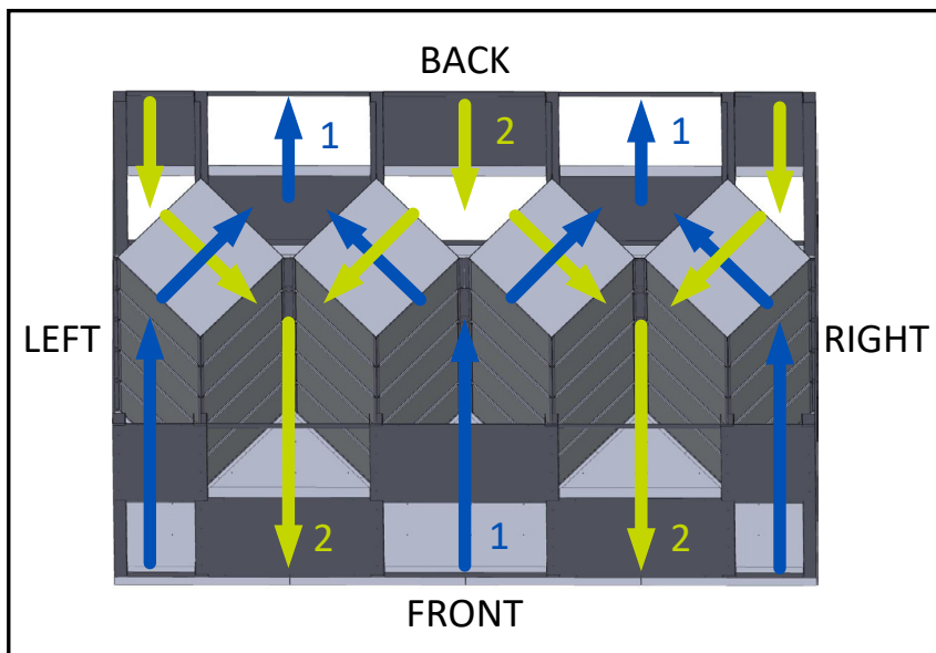
FIGURE 2.0.0 CROSSFLOW OPPOSITE SIDE ARRANGEMENT 1
