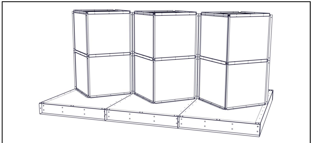
FIGURE 5.4.1 CORE STACKING
