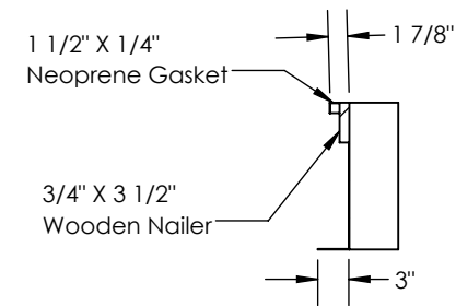
CURB CROSS-SECTION A-A (TYP.)
