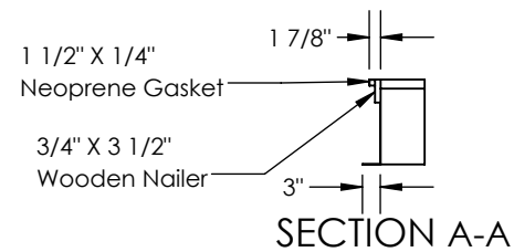
CURB CROSS-SECTION A-A (TYP.)
