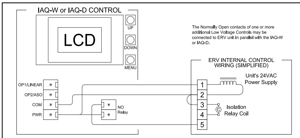
FIGURE 3.1.3 WIRING SCHEMATIC FOR LE-SERIES, AND ALL HE3X AND LARGER UNITS WITHOUT VFDS OR ECM
