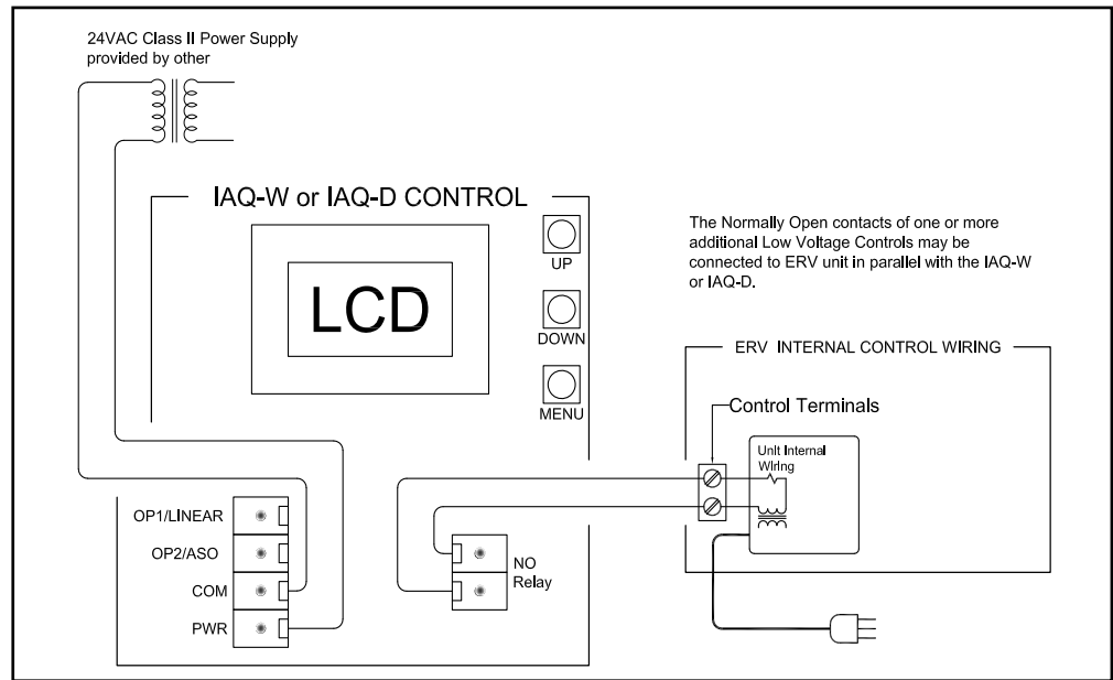
FIGURE 3.1.0 WIRING SCHEMATIC FOR EV90, EV130, EV200 UNITS ONLY
