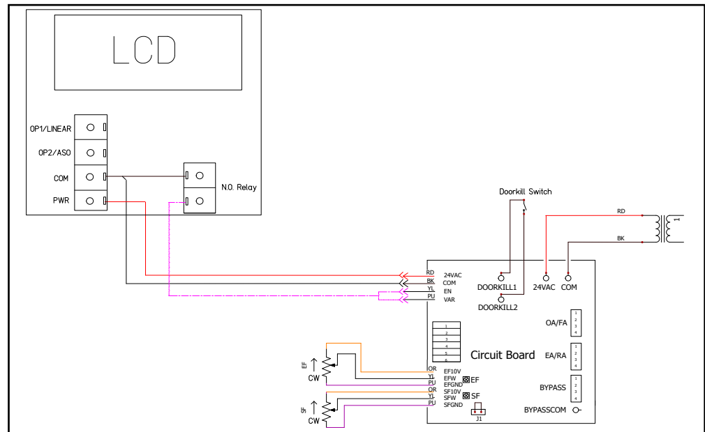
FIGURE 3.1.5 WIRING SCHEMATIC FOR HE05, HE07, HE10, HE15, AND HE20 UNITS WITH ECM AND CIRCUIT BOARD
