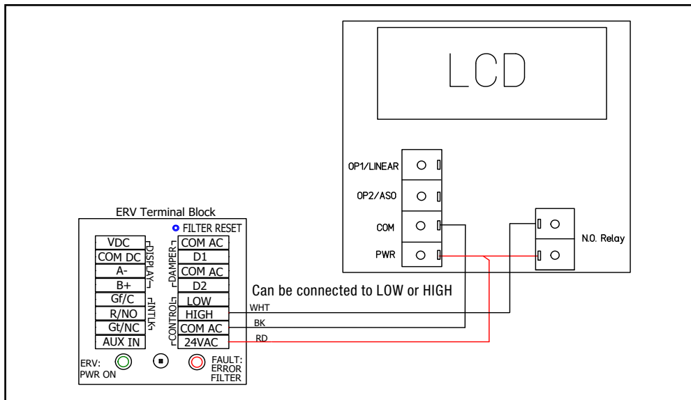
FIGURE 3.1.2 WIRING SCHEMATIC FOR EV PREMIUM+ AND SL+ 75 UNITS
