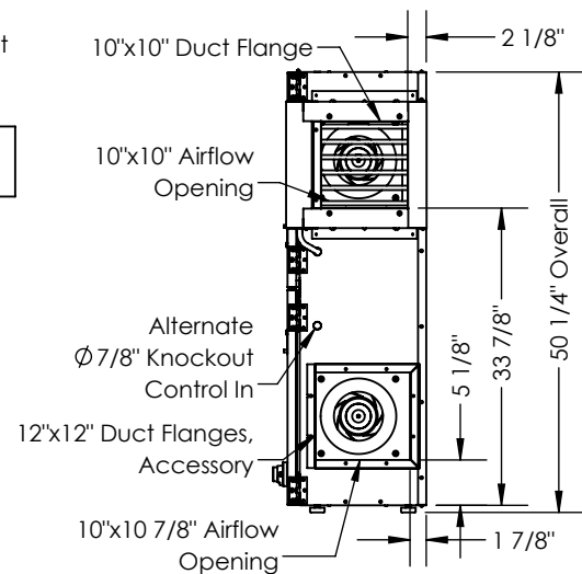
RIGHT VIEW
